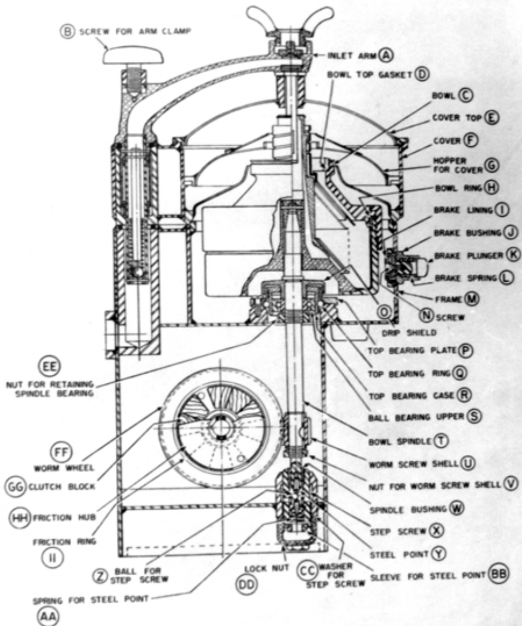
VERTICAL SECTION THRU SPINDLE
