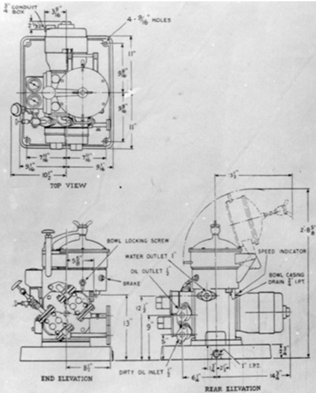
GENERAL DIMENSIONS
