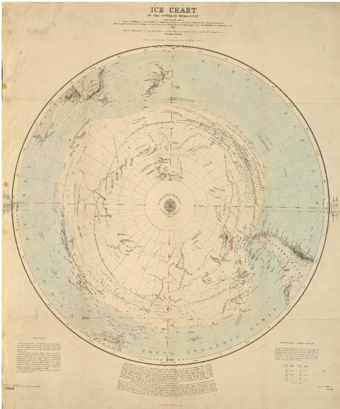
Ice chart of the Southern hemisphere [material cartográfico] Hydrographic Office Admty.
